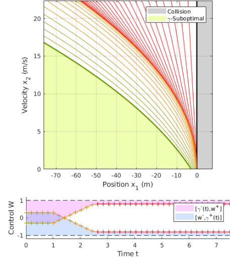
Fig. 2: Top: Computed suboptimal safety set \text{Sub}_T^{\gamma^-(\cdot), \gamma^+(\cdot)} for the braking scenario. The contour curves represent constant \theta(x) = t (or \varphi(t, x) = 0 ) for times 0.2s apart. Bottom: The suboptimal control parameterization. Lines are \gamma^-(\cdot), \gamma^+(\cdot) , and the plus markers correspond to contour lines in the top figure. Colors delineate the three modes defined in Section V.
