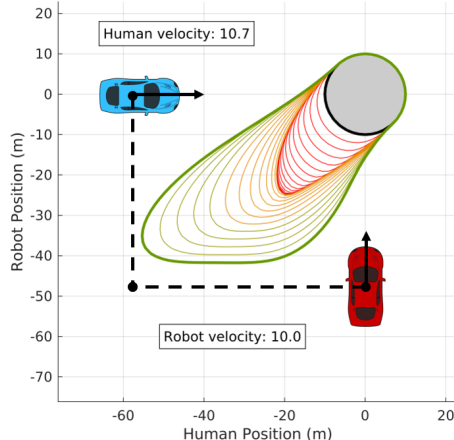
Fig. 1: Computed suboptimal safety set \text{Sub}_T^{\gamma^-(\cdot), \gamma^+(\cdot)} for the intersection problem, the states outside of the thick green line.
