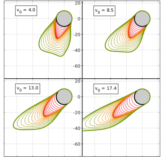
Fig. 5: Slices of the intersection scenario state space for various human velocities.
