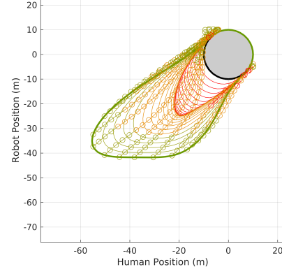
Fig. 6: Simulating worst-case trajectories for the intersection scenario by sampling x_0 \in \partial \text{Sub}_T^{\gamma^-(\cdot), \gamma^+(\cdot)} and executing worst-case closed loop control trajectories.
