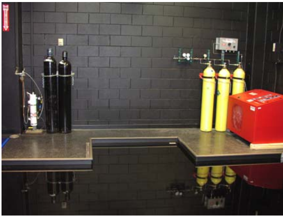
(a) A view of the compressed air filling system.
